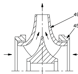
Fig. 16 Double-suction impeller
