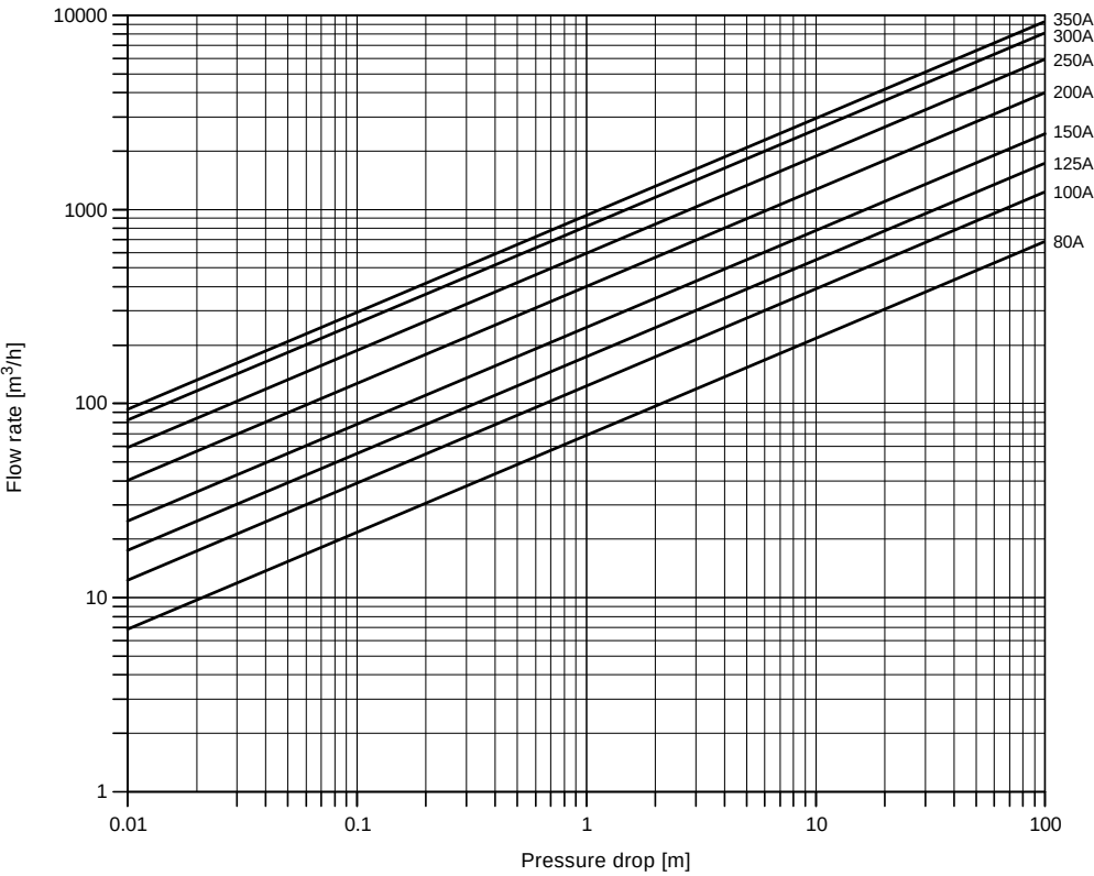
Fig. 43 Pressure drop graph for suction diffusers. The designation of the lines, such as “100 A”, refers to the DN size of the outlet flange.
