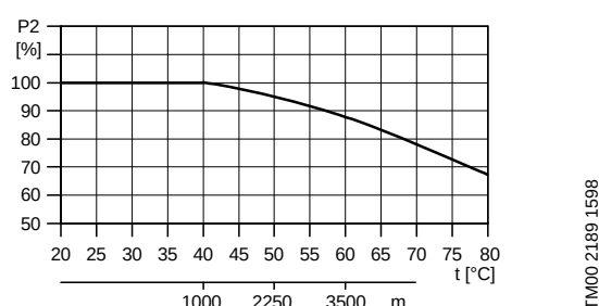
Fig. 21 Relationship between motor output (P2) and ambient temperature
