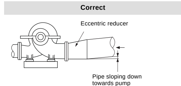
Fig. 28 Correctly mounted suction piping
