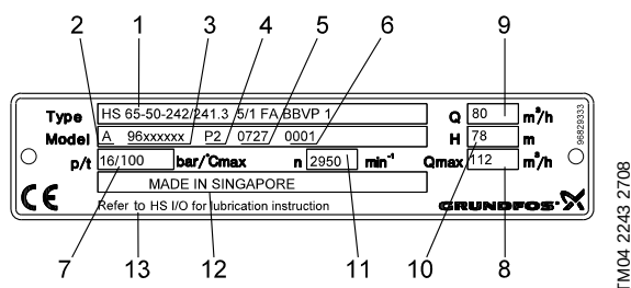
Fig. 7 Nameplate of HS pump version 5
