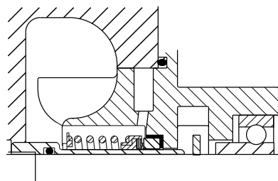
Fig. 18 Rubber bellows shaft seal, type B
